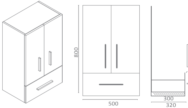
COLGAR CAJÓN WALL DRAWER UNIT ARMOIRETTE TIROIR
