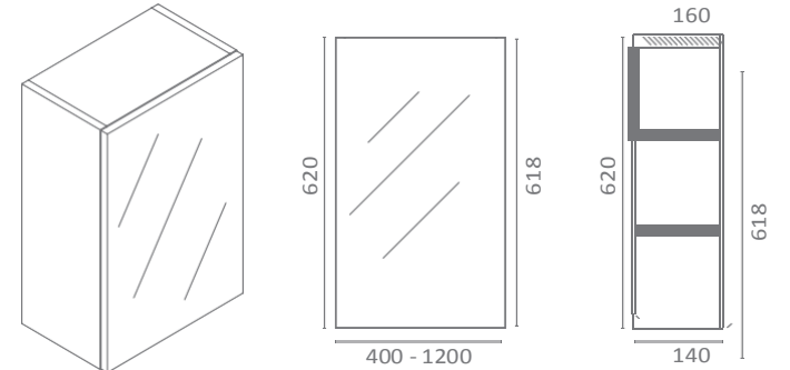
CAMERINO MIRROR WALL UNIT ARMOIRETTE MIROIR
