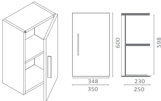
COLGAR WALL UNIT ARMOIRETTE
