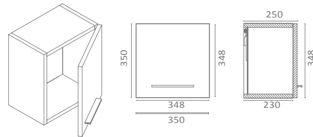
COLGAR WALL UNIT ARMOIRETTE
