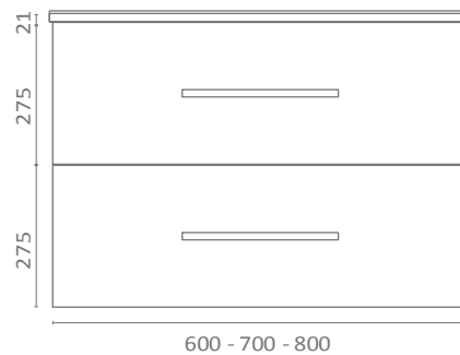
FRONTAL FRONT SIDE FAÇADE
