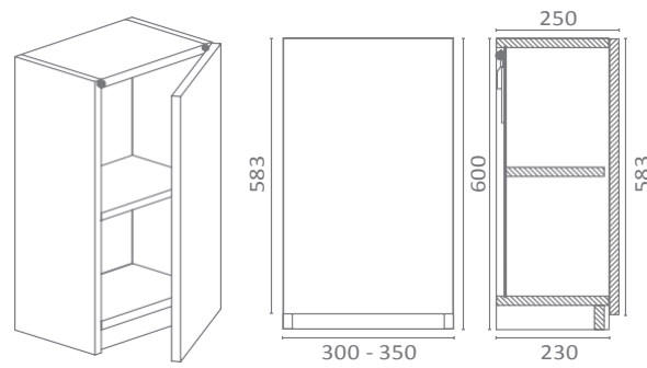
COLGAR UÑERO WALL HANDLESS UNIT ARMOIRETTE PRISE DE MAIN
