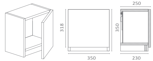
COLGAR UÑERO WALL HANDLESS UNIT ARMOIRETTE PRISE DE MAIN
