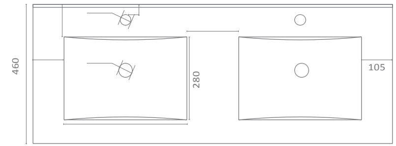
2 SENOS / 2 BOWLS / VASQUE DOUBLE
