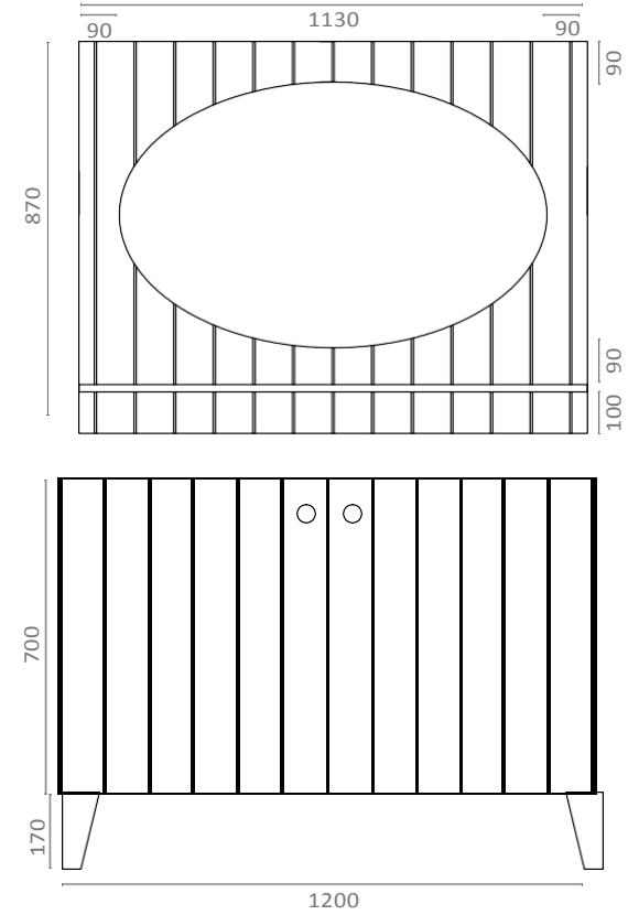
FRONTAL FRONT SIDE FAÇADE
